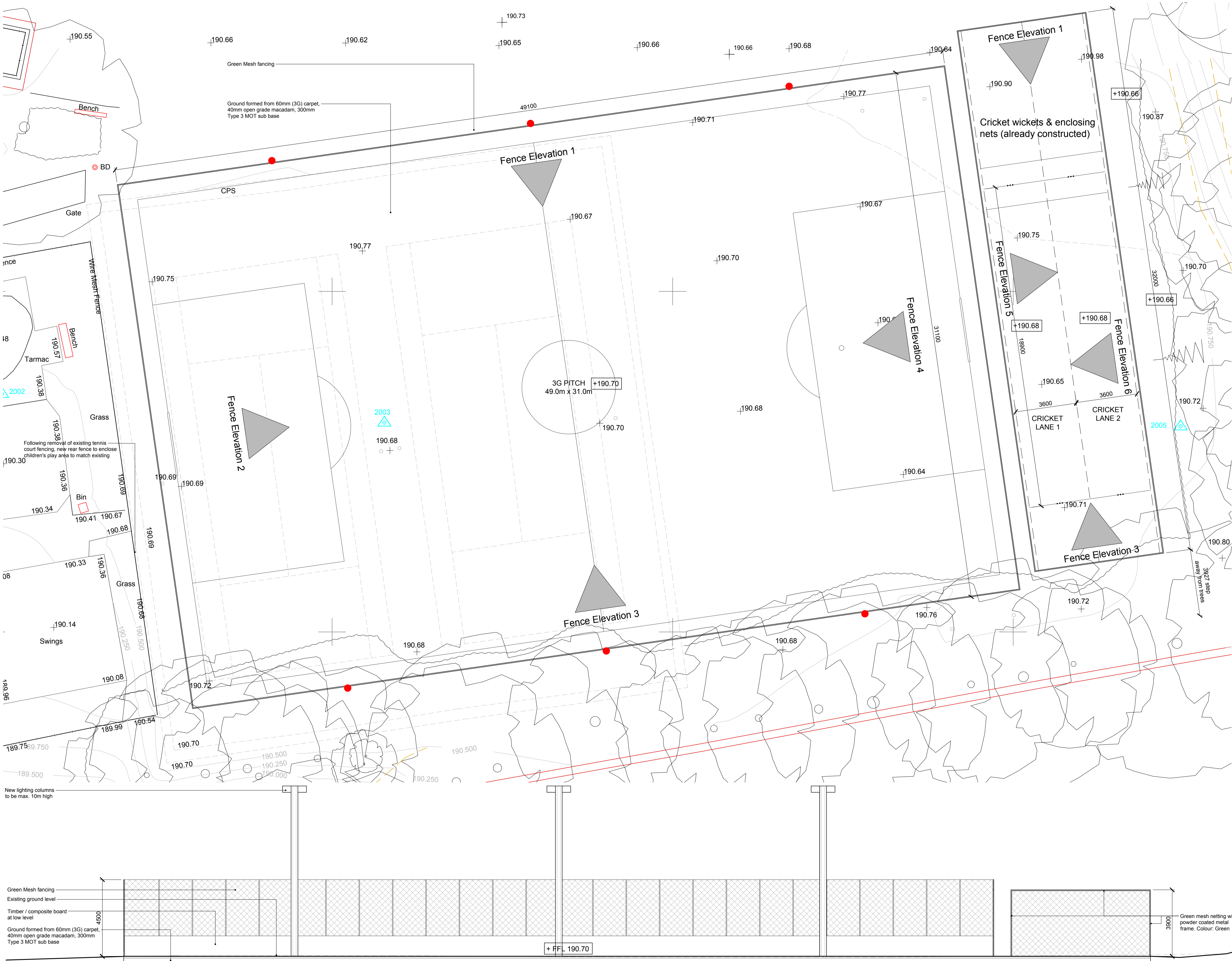
Back Fence Elevation To 3G Pitch & Cricket Nets (Elevation 3)
